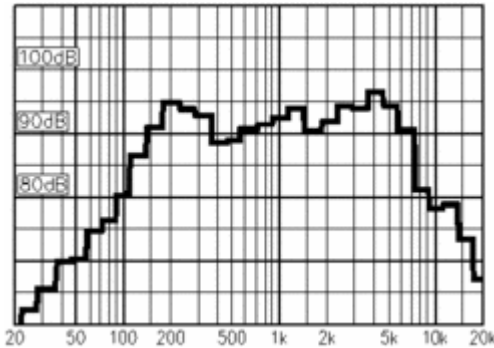
1W/1m Pink Noise 1/3 octave bands.
